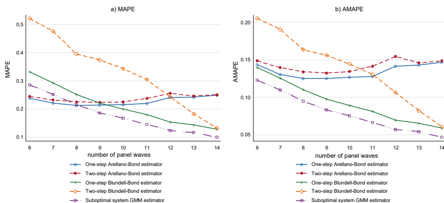
Figure –12. Relative prediction error measures of the parameter \rho (MAPE, AMAPE) for the different estimation methods as a function of the number of T panel waves.
